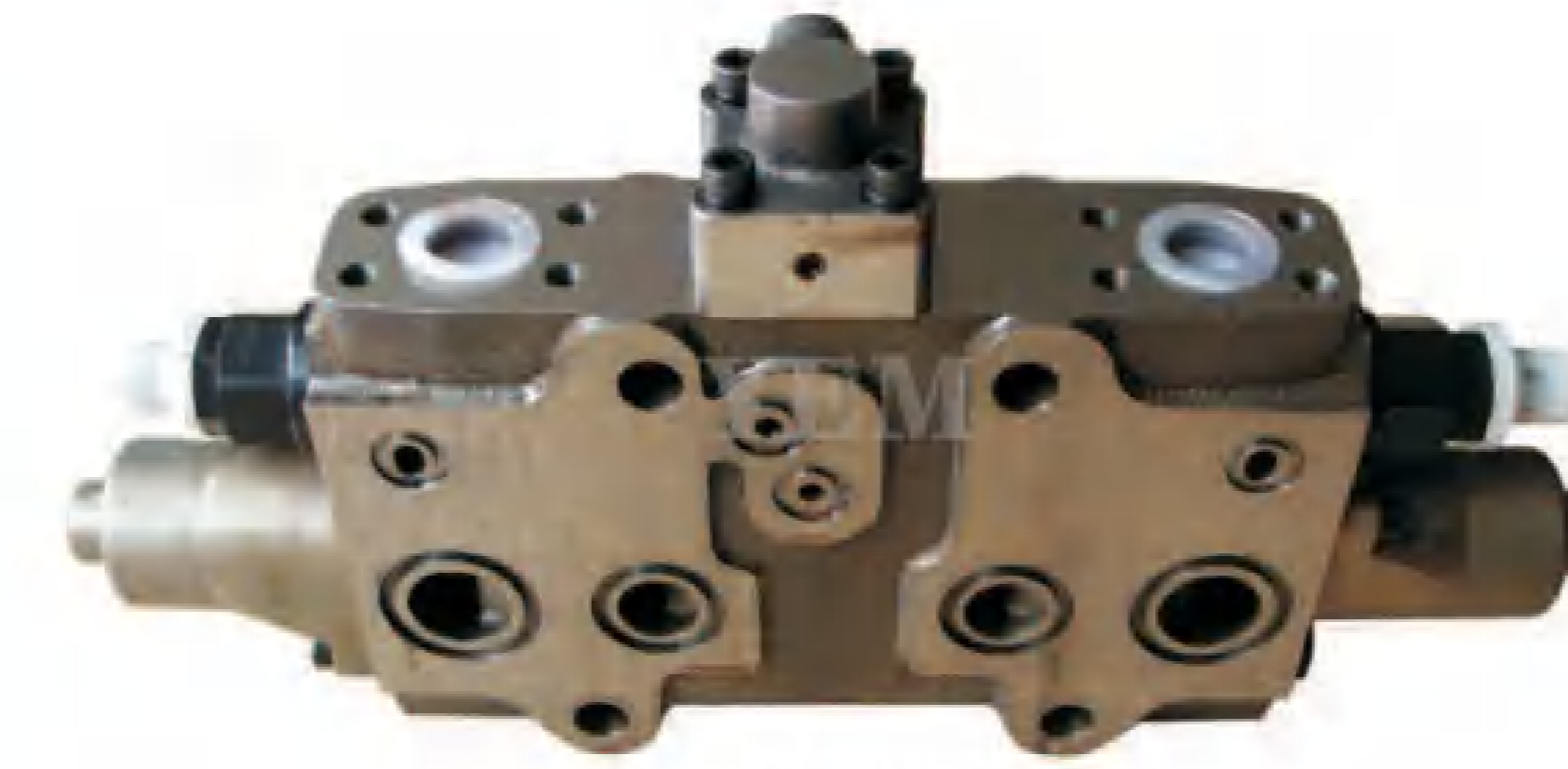
YEM-H7587 PC200-7 PC220-7 723-41-07600备用阀 Standby valve hydraulic hammer
